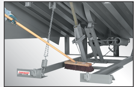
CleanSweep Frame allows unobstructed access to the pit area.
